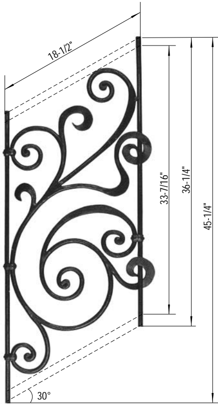
Art.4022 H.45-1/4"xL.16-9/16" ●9/16"
